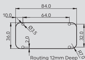
Recessed handle - 90mm
