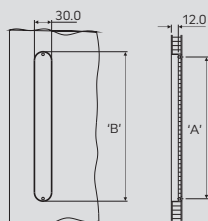
Shutter Handle - Al. 3012
