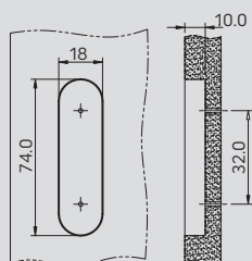
Concealed Hook Handle
