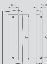
Shutter Handle - Al. 3012 Square
