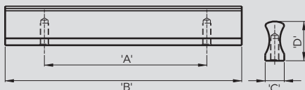
Al. Handle - I1 Finish: SL/SF/BA
