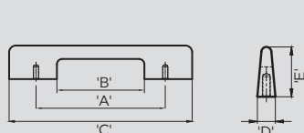
Al. Handle - C4-2 Finish: BA/AB/SF
