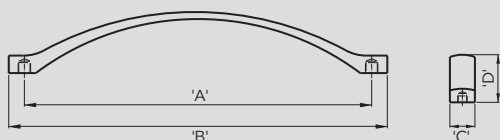
Zinc Handle - A1 Finish: NB
