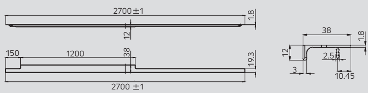
Edge Profile Handle - 1 (L/R) Finish: SF/AB
