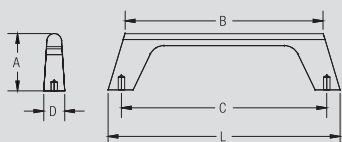
Zinc Handle - C1 Finish: NB
