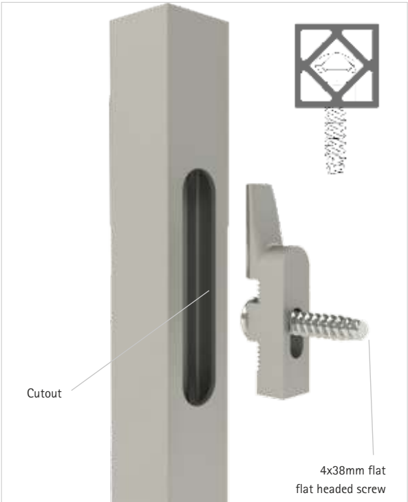
Cutout Dimensions: 11mm x 55 mm (top & bottom with 11 mm dia round)
