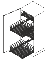
For carcase width 600 mm
