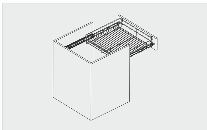
5. Final assembly, basket fixed to fascia
