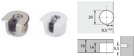
Dowel centre from underside of shelf
