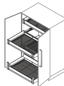
For carcase width 900 mm
