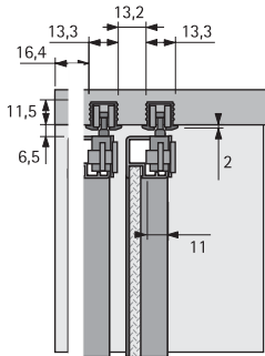
For aluminium framed doors
