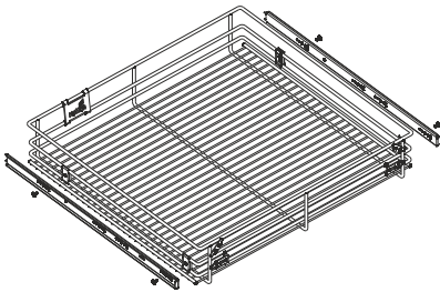
2. Attach clips
