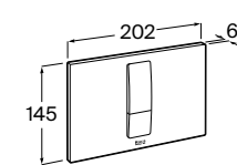
Stainless Steel Ref. A890221304
