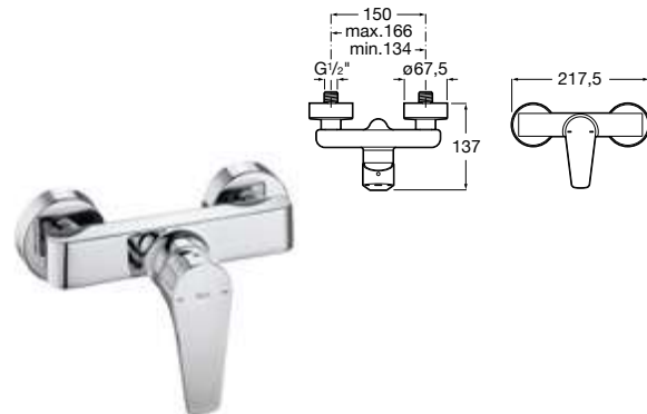
Single-lever shower mixer. Chrome. Ref. A5A2190C00
