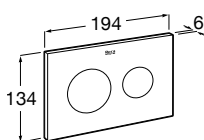
Stainless Steel Ref. A890223304
