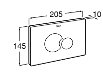
Chrome Ref. A890222301 White Matt Ref. A890222307
