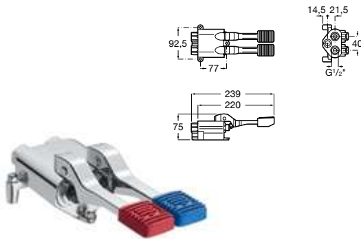
Foot pedal, self-closing mixer. Floor-mounted. Ref. A505128600
