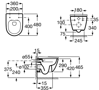
SUPRALIT® seat and cover, metal hinges Ref. A801E20..1
