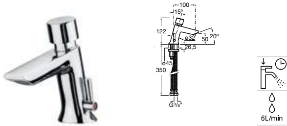
Basin mixer with aerator. G3/8". Flow: 6 l/m. Automatic closing: 15 sec. Chromed. Ref. A5A3177C00
