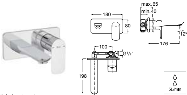
Built-in basin mixer. Chrome Ref. A5A356EC00
