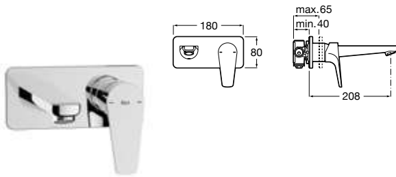
Built-in basin mixer. Chrome. Ref. A5A3590C00
