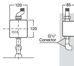
Built-in part, connection to mains. Ref. A525165303
