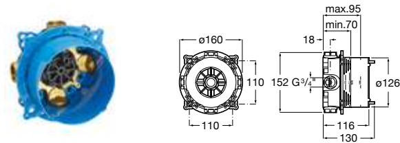
RocaBox Universal. Ref. A525869403
