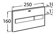
Plate PL7 Dual Operating plate Matt black Ref. A890088206
