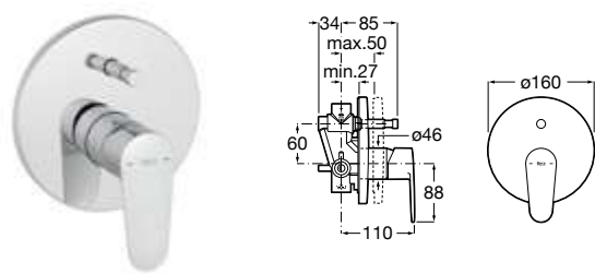
Single-lever built-in bath-shower mixer with automatic diverter. Chrome. Ref. A5A064FC00
