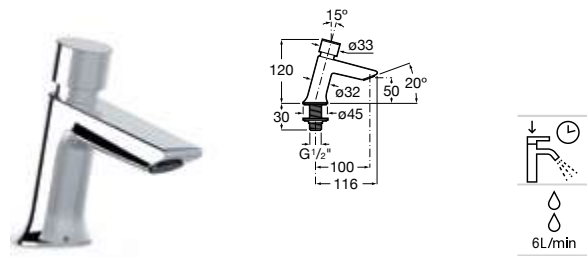
Basin faucet with aerator. G1/2". Flow: 6 l/m. Automatic closing: 15 sec. Chromed. Ref. A5A4277C00
