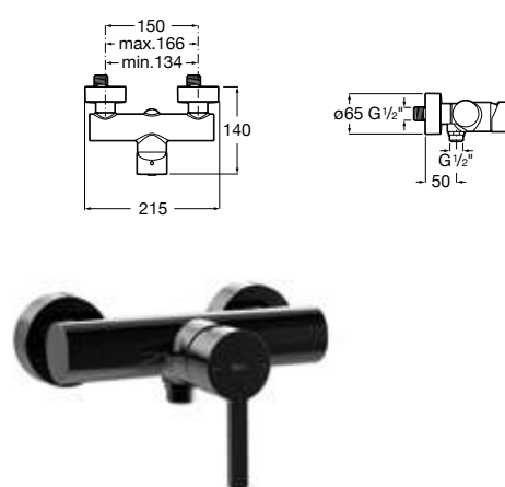
Single-lever shower mixer Everlux. Ref. A5A2196..0
