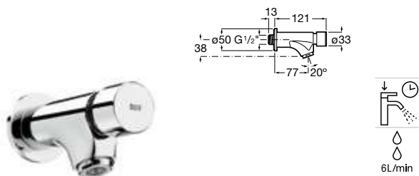
Wall-mounted basin faucet with aerator G1/2". Flow: 6 l/m. Automatic closing: 15 sec Chromed. Ref. A5A7877C00
