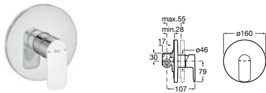
Single-lever built-in bath or shower mixer Chrome Ref. A5A226EC00
