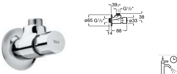
Shower faucet. Angle shut-off cock. G1/2". Chromed. Ref. A5A2777C00
