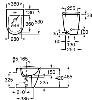
SUPRALIT® cover for bidet Ref. A806E10..1
