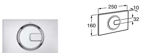
Plate PL4.A Dual Operating plate Chrome Ref. A890198001
