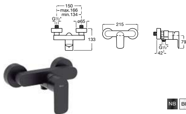
Single-lever shower mixer. Ref. A5A216E..0
