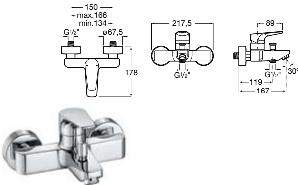
Single-lever bath-shower mixer with automatic diverter. Chrome. Ref. A5A0290C00
