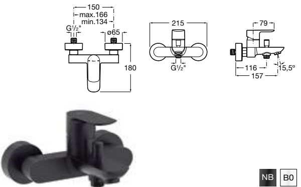
Single-lever bath-shower mixer with automatic diverter. Ref. A5A026E..0
