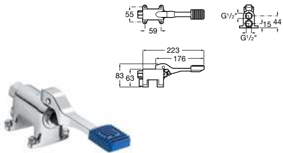
Foot pedal, self-closing, one water. Floor-mounted. Ref. A505127800
