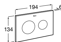
Chrome Ref. A890223301 White Matt Ref. A890223307
