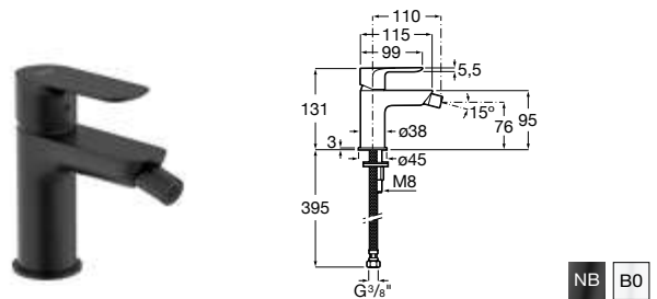
Single-lever bidet mixer with aerator and flexible supply hoses. Ref. A5A626E..0
