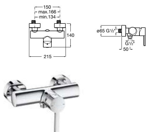
Single-lever shower mixer Chrome. Ref. A5A2196C00
