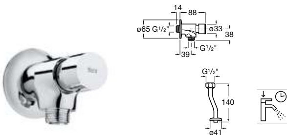
Urinal faucet. Angle shut-off cock G1/2" Chromed. Ref. A5A9277C00
