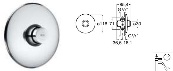
Shower faucet. Built-in shut-off cock. G1/2. Chromed. Ref. A5A2677C00
