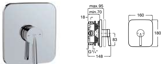
Built-in bath or shower mixer. Chrome. To completed with RocaBox A525869403. Ref. A5A2B6DC00
