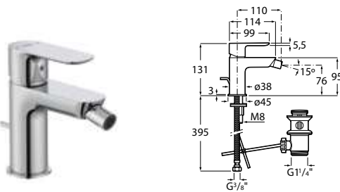
Single-lever bidet mixer with aerator, pop-up waste and flexible supply hoses. Chrome Ref. A5A606EC00
