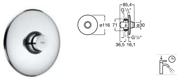
Urinal faucet. Built-in shut-off cock. G1/2. Chromed. Ref. A5A9077C00
