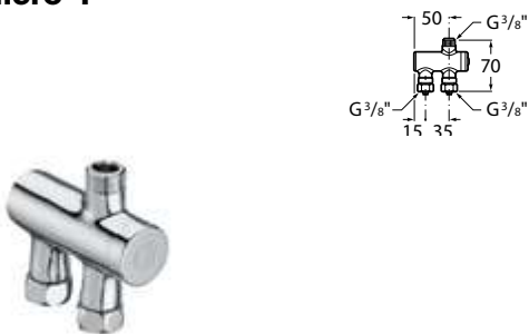
Thermostatic Micro-T Premixed water. Chrome. Ref. A5A0179C00
