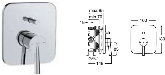
Built-in bath-shower mixer with automatic diverter. Chrome. To be completed with RocaBox A525869403 Ref. A5A0B6DC00
