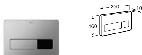
Plate PL3.A Dual Electronic Electronic stainless steel operating plate for concealed cistern with automatic or manual dual flush Ref. A890097500
